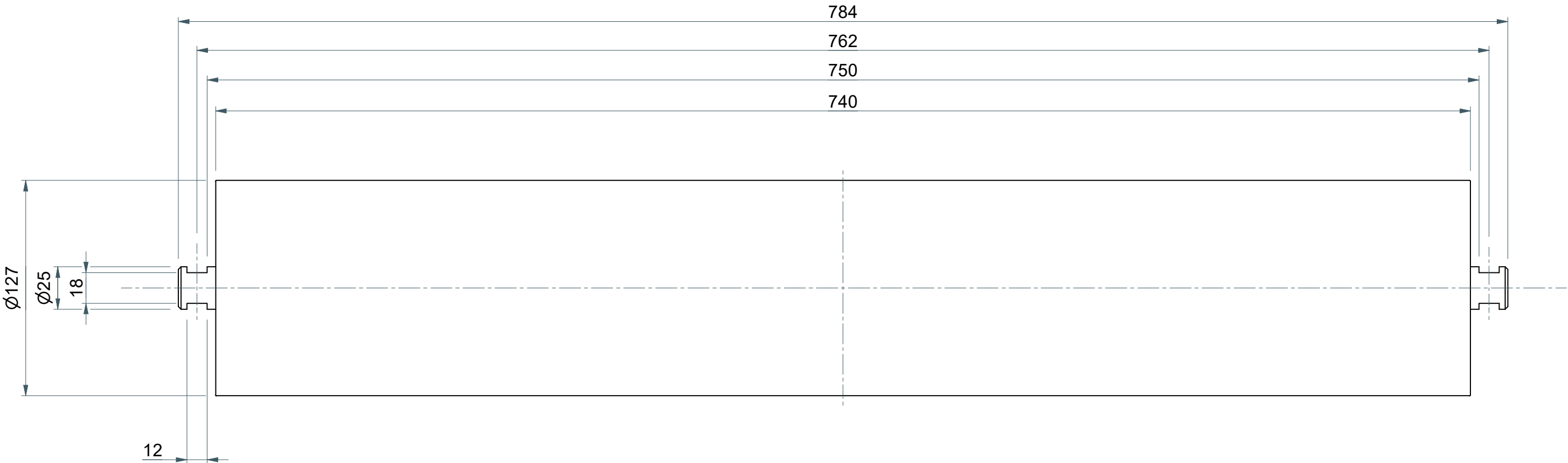
PLAN VIEW SCALE: 1 : 2.5
