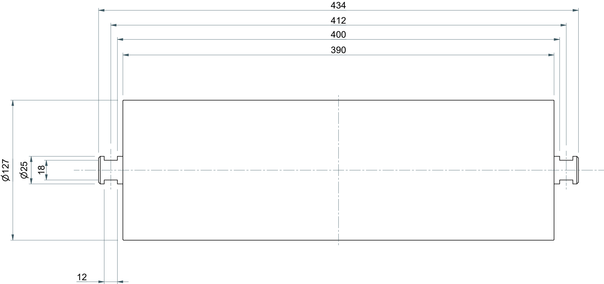
PLAN VIEW SCALE: 1 : 2
