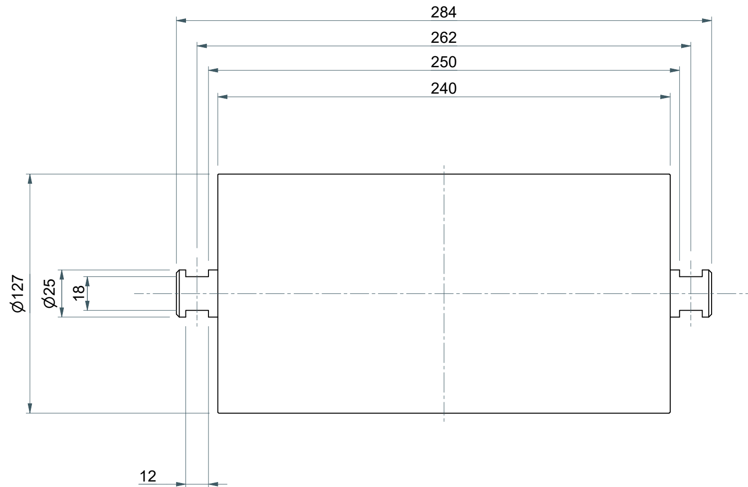
PLAN VIEW SCALE: 1 : 2
